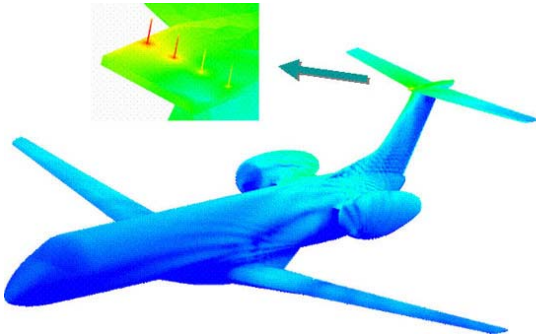
Figure 1: Surface currents from excitation of monopole no. 1
