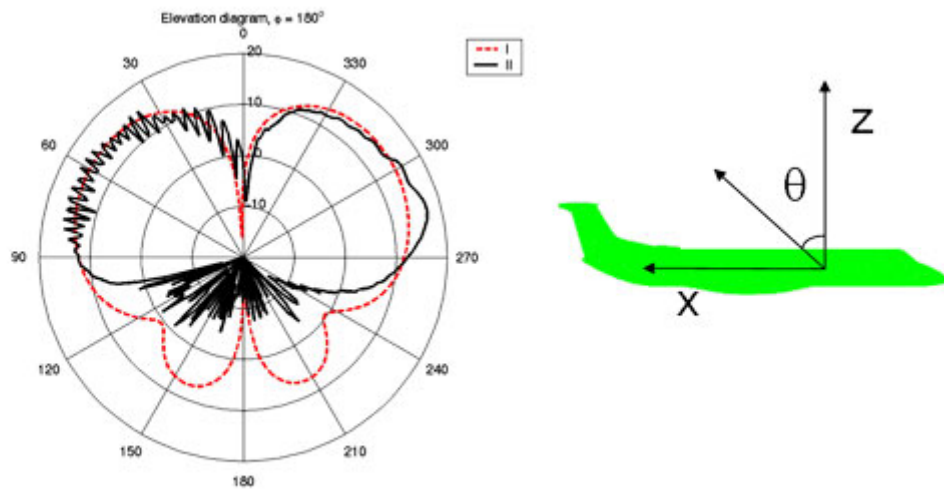
Figure 2: Elevation diagram example
